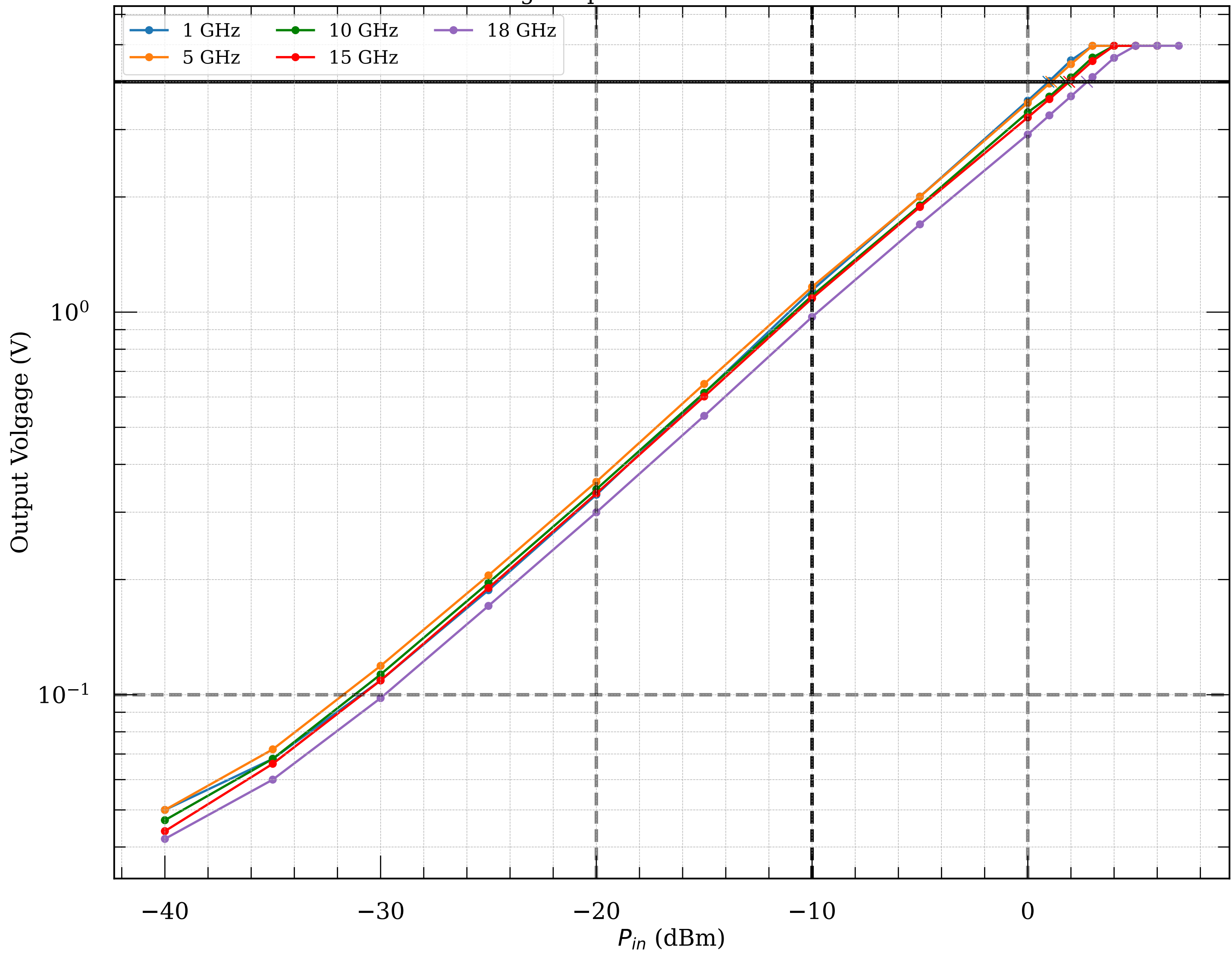
Measured voltage-to-power curve of detector module100
